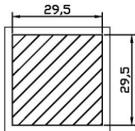
Thermal pad 29.5 x 29.5 mm
